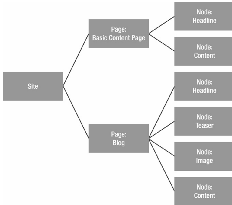
Figure 5-1. The content node pattern
