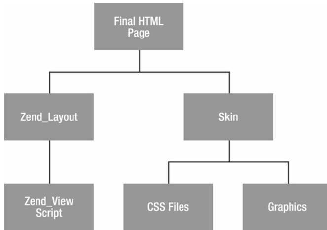
Figure 2-1. Three-step views with Zend_View, Zend_Layout, and skins
