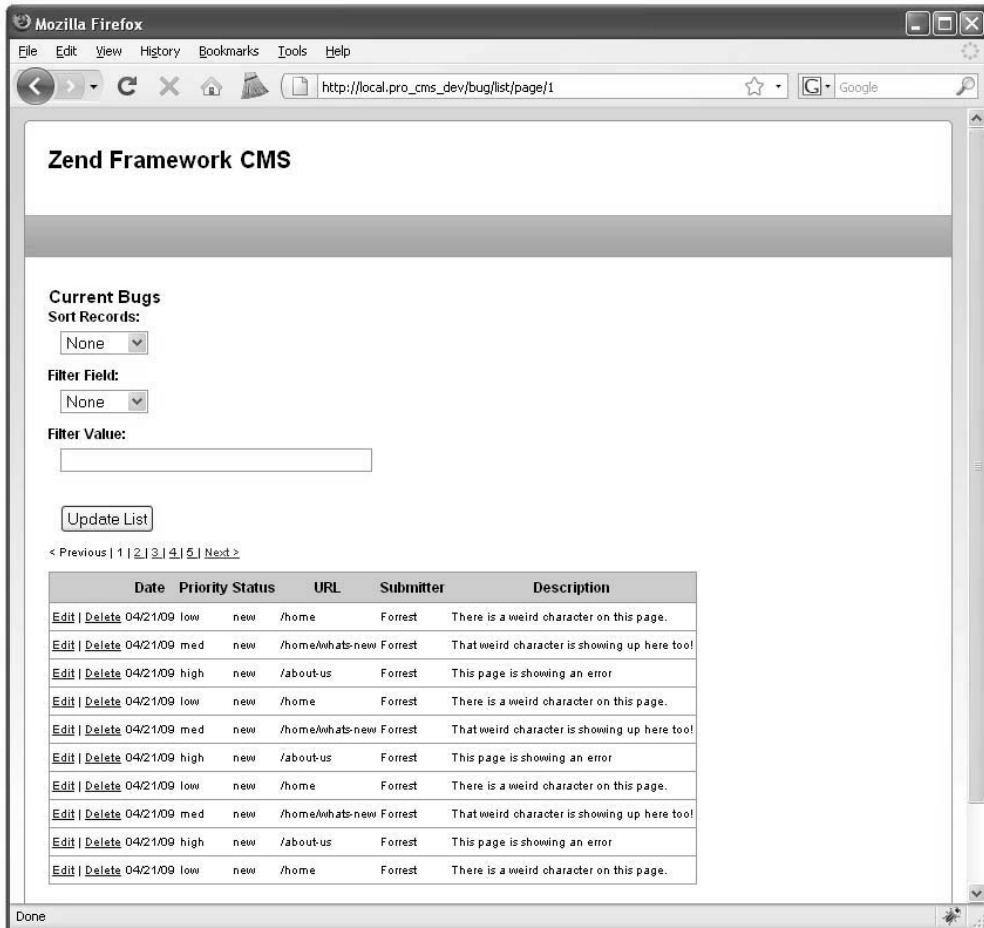
Figure 4-2. The completed list view
